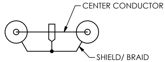
SCHEMATIC DIAGRAM
